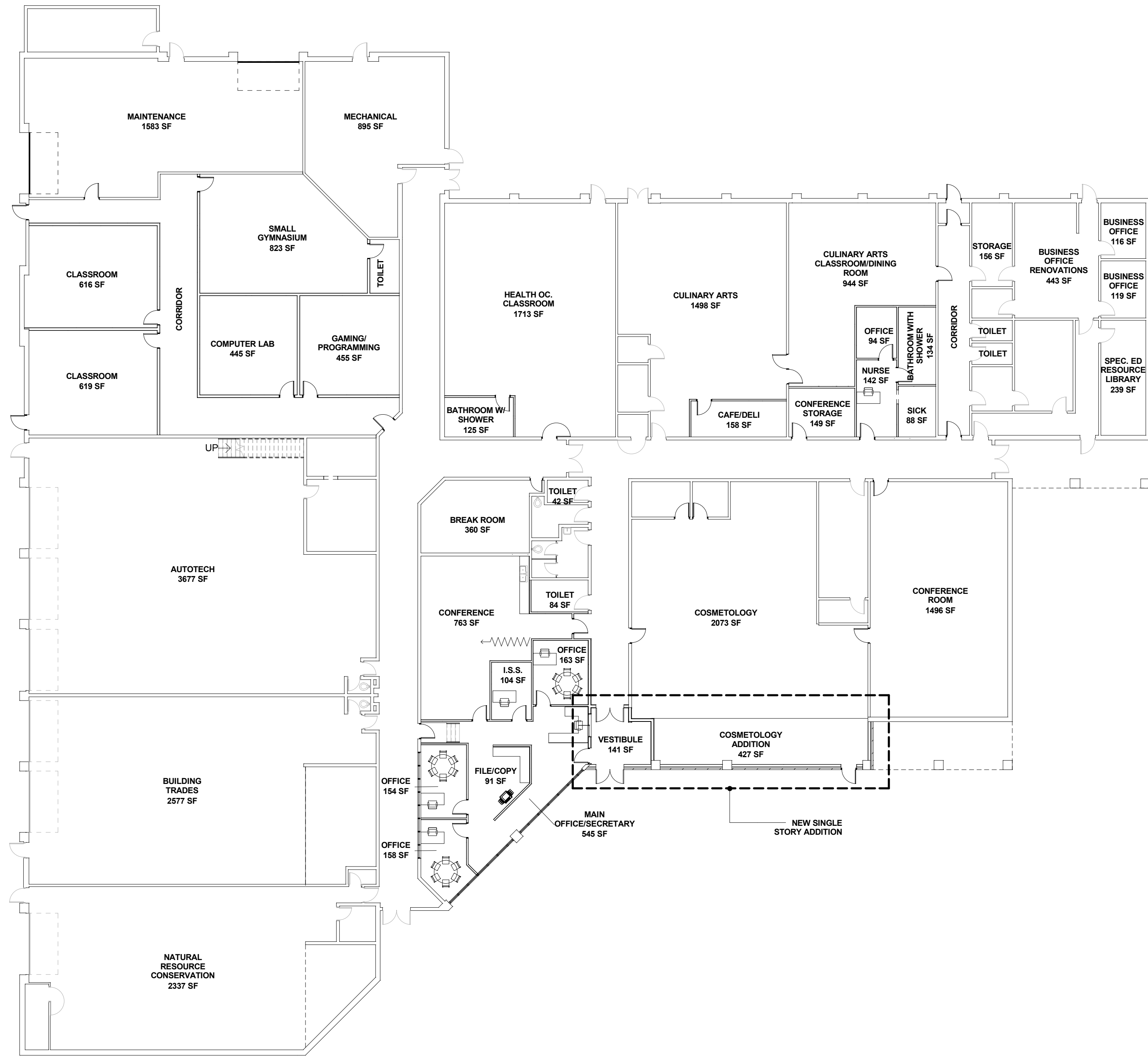
FIRST FLOOR PLAN SCALE: 1/16" = 1'-0"
